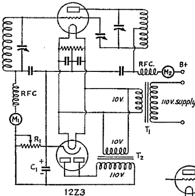
FIG. 1—CIRCUIT OF THE TRANSMITTER BIAS SUPPLY
